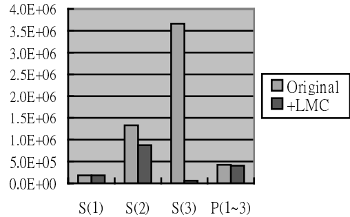
Figure 1: The number of different types of syllable-based indexing terms before or after applying the language model constraints for pruning.
