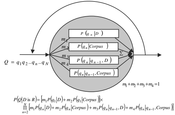
Figure 1: The HMM structure for a specific document D .
